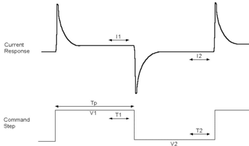
Figure F-0-1. MT Command Pulse & Response
